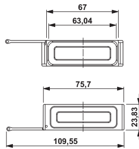
Dimensional drawing
