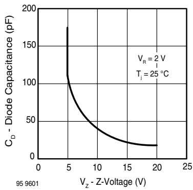
Figure 6. Diode Capacitance vs. Z-Voltage
