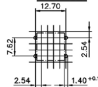
PCB lead
