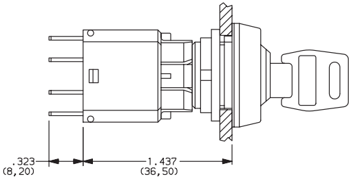
Standard Contact Block with Momentary or Latching Switchlock
