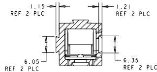
SECTION N-N
