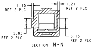
SECTION N-N
