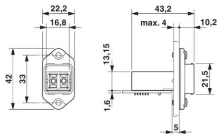
Push-Pull SCRJ panel mounting frame
