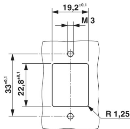
Panel cutout
