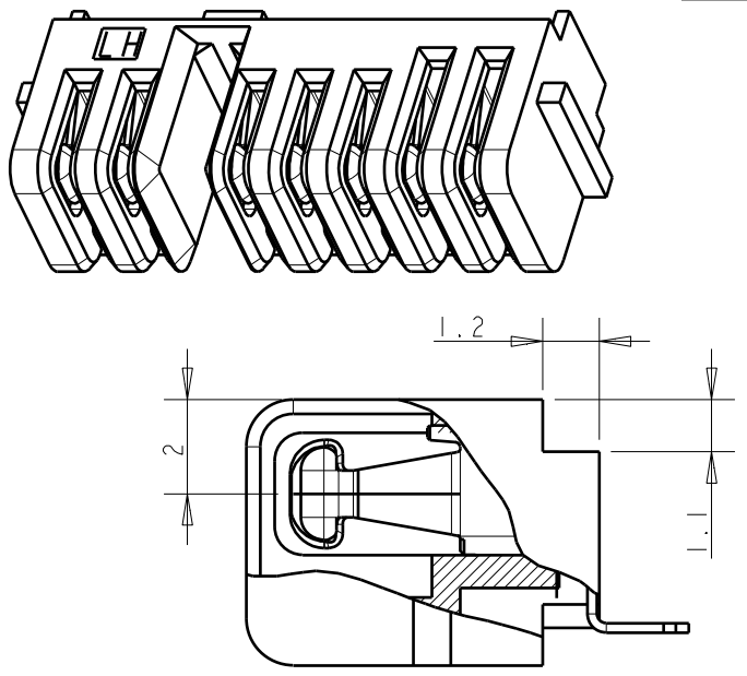
SECTION A-A SCALE 6:1
