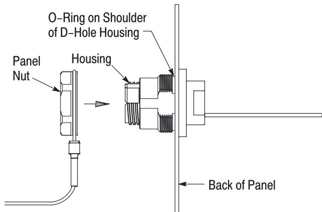
Detail A
