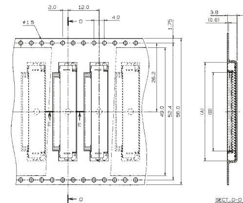
SECT. D-D
