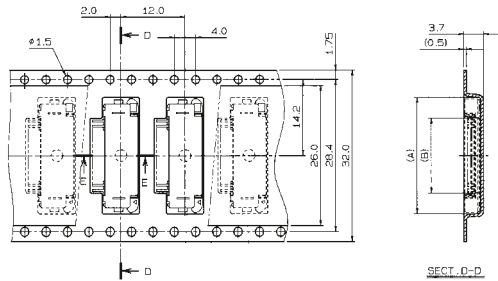
SECT. D-D
