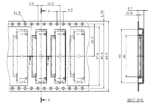
SECT. D-D
