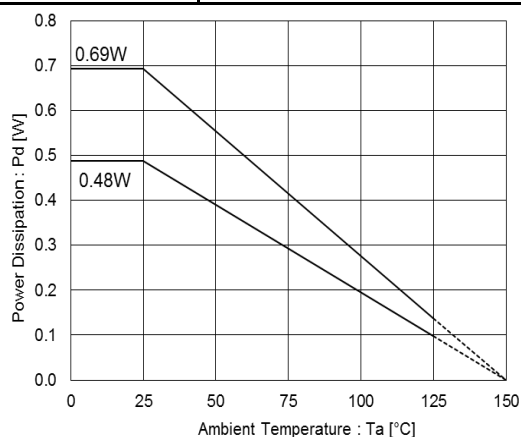
Figure 29. SS0N004R1010 Power dissipation heat reduction characteristics (Reference)
