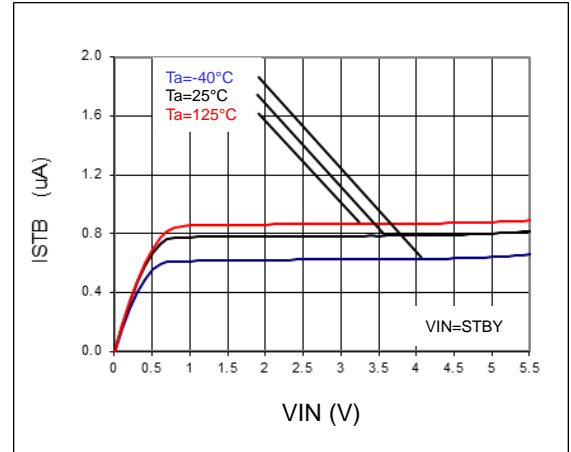
Figure 6. VSTBY - ISTB
