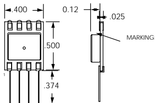
No Pressure Port BARO-A-PRIME-MINI
