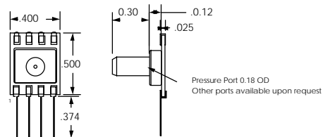
Single Pressure Port BARO-AF-PRIME-MINI
