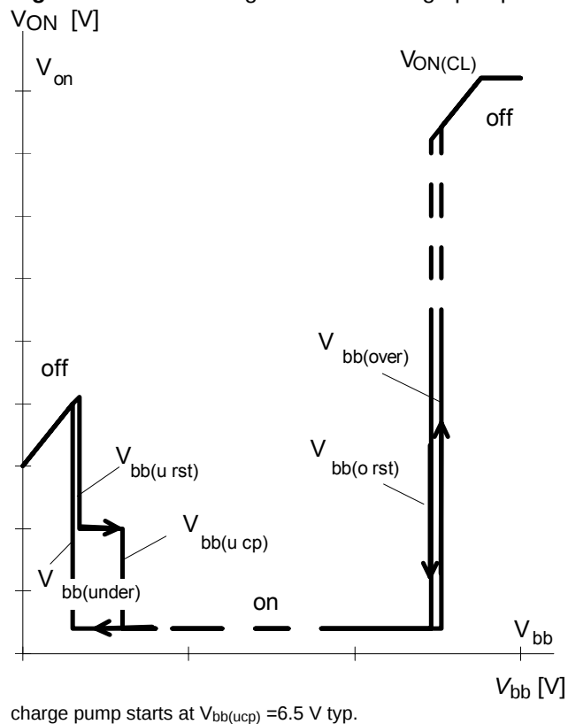
Figure 7a: Overvoltage:
