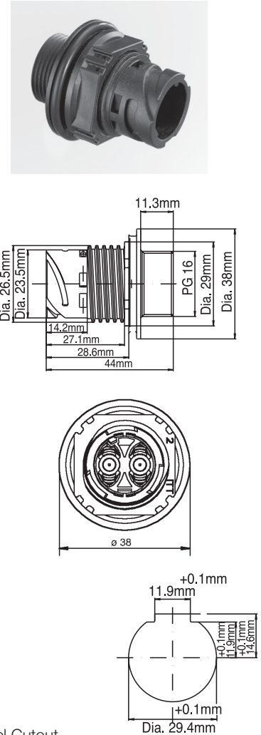
Panel Cutout Panel Thickness 4mm Max. / .8mm Min.
