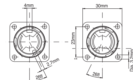
Panel Cutout Panel Thickness 3mm Max.
