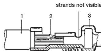
Incorrect Crimp
