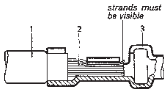
Correct Crimp
