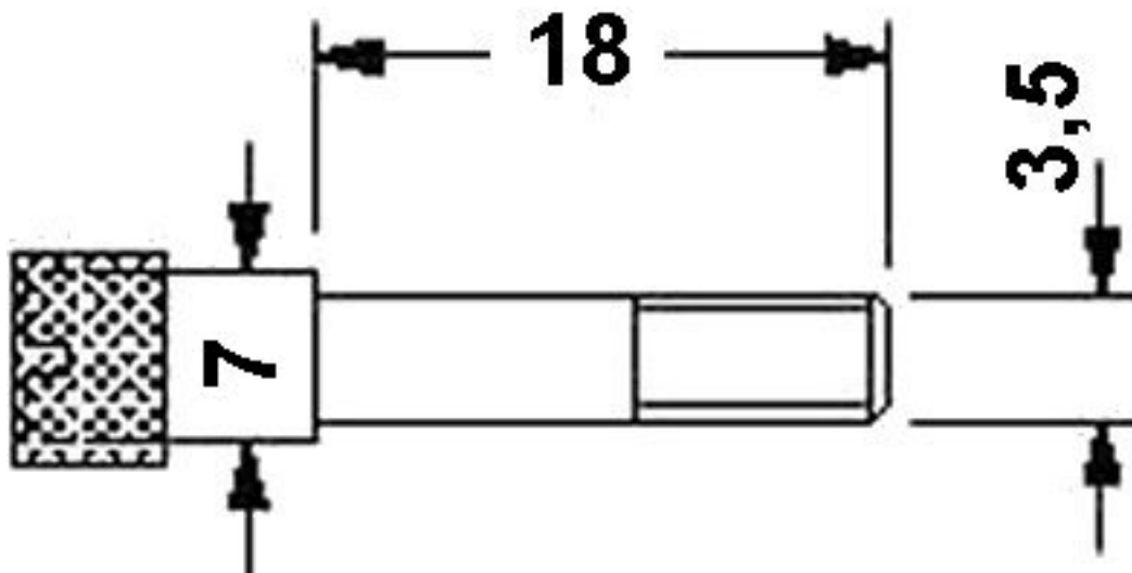
Dimensioned drawing
