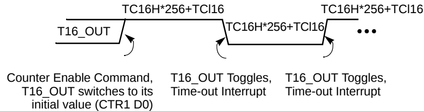
Figure 41. T16_OUT in Modulo-N Mode
