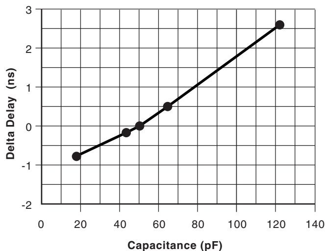
Figure 35: Delay Factor at Various Capacitive Loads
