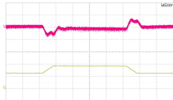
Fig. 11: Output voltage response to load current step change (24A – 36A – 24A) at V_{in} = 48\text{ V} . Top trace: output voltage (200mV/div.). Bottom trace: load current (20 A/div.). Current slew rate: 0.1 A/ \mu\text{s} . C_o = 1\mu\text{F} ceramic + 10 \mu\text{F} tantalum. Time scale: 200 \mu\text{s} /div.
