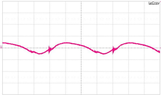
Fig. 13: Output voltage ripple (50 mV/div.) at full rated load current C_o = 10 \mu\text{F} tantalum + 1 \mu\text{F} ceramic and V_{in} = 48 \text{ V} . Time scale: 1 \mu\text{s}/\text{div} .
