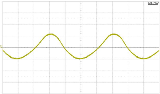
Fig. 15: Input reflected ripple current, i_c (1 A/div.), measured at input terminals at full rated load current and V_{in} = 48 \text{ V} . Refer to Fig. 14 for test setup. Time scale: 1 \mu\text{s}/\text{div} .
