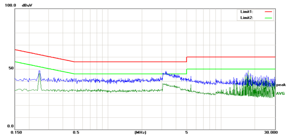
Fig. 19: Vin+ Peak Detector EMI waveform
