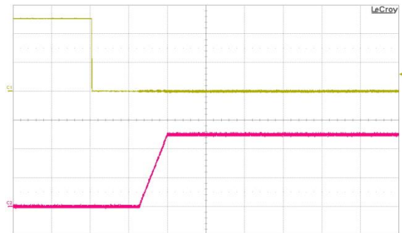
Fig. 10: Turn-on transient at full rated load current (resistive) plus 6000 \mu\text{F} at V_{in} = 48\text{ V} , triggered via ON/OFF pin. Top trace: ON/OFF signal (2V/div.). Bottom trace: output voltage (2V/div.). Time scale: 50 ms/div.
