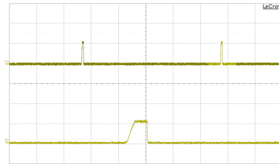
Fig. 17: Load current (top trace, 50 A/div., 100 ms/div.) into a 10\text{m}\Omega short circuit during restart, at V_{in} = 48 \text{ V} . Bottom trace (50 A/div., 10 ms/div.) is an expansion of the on-time portion of the top trace
