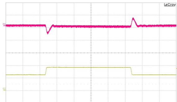
Fig. 12: Output voltage response to load current step change (24 A – 36A – 24 A) at V_{in} = 48\text{ V} . Top trace: output voltage (500mV/div.). Bottom trace: load current (10A/div.). Current slew rate: 1A/ \mu\text{s} . C_o = 1\mu\text{F} ceramic + 6000 \mu\text{F} + 10 \mu\text{F} tantalum. Time scale: 200 \mu\text{s} /div.
