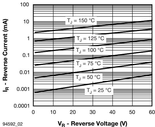
94592_02 Fig. 2 - Typical Peak Reverse Current vs. Reverse Voltage
