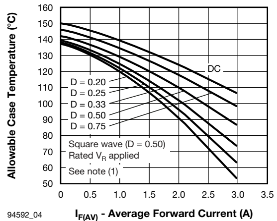
94592_04 Fig. 4 - Maximum Average Forward Current vs. Allowable Lead Temperature
