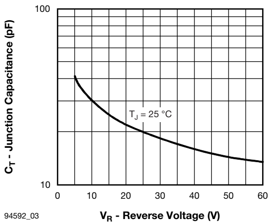
94592_03 Fig. 3 - Typical Junction Capacitance vs. Reverse Voltage
