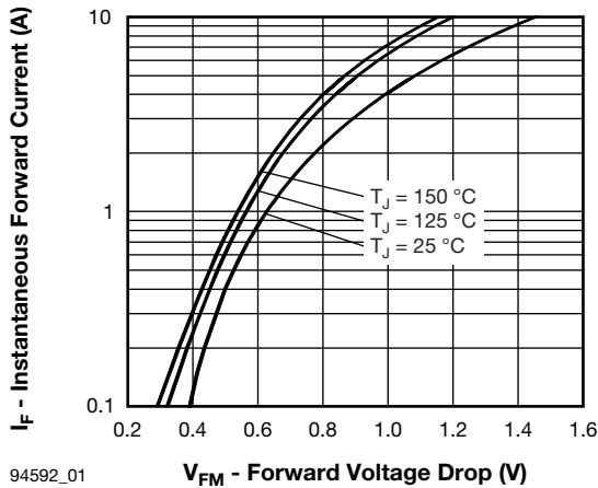
94592_01 Fig. 1 - Maximum Forward Voltage Drop Characteristics
