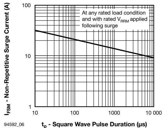
94592_06 Fig. 6 - Maximum Peak Surge Forward Current vs. Pulse Duration
