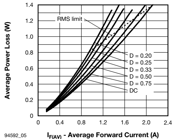
94592_05 Fig. 5 - Maximum Average Forward Dissipation vs. Average Forward Current
