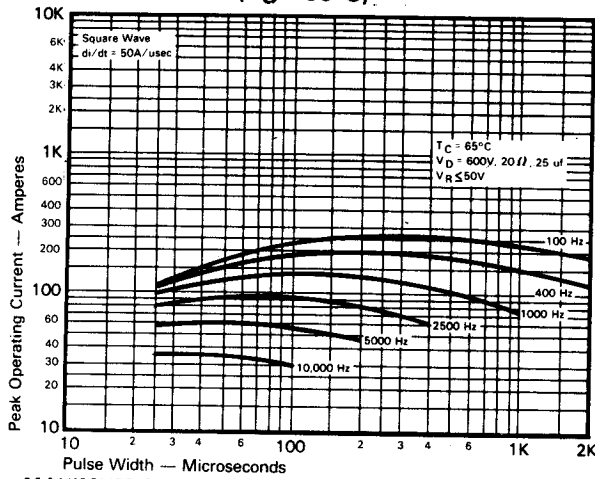
MAXIMUM ALLOWABLE PEAK ON-STATE CURRENT vs. PULSE WIDTH ( di/dt = 50\text{A/us} )
