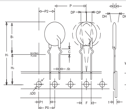
TMOV varistor with outer crimp
