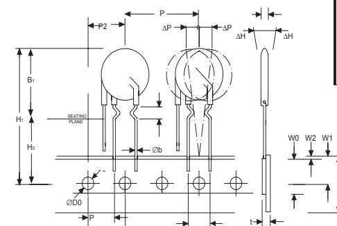
iTMOV varistor with inner crimp
