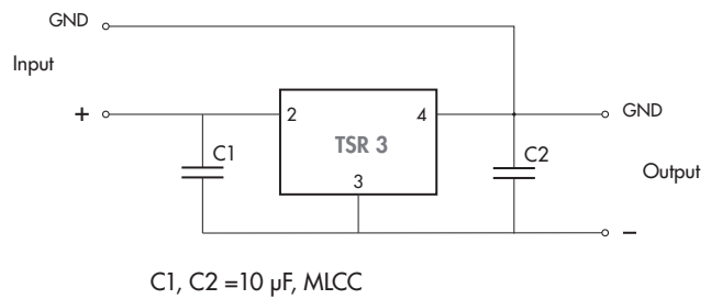
fig. 2 Negative output circuit
