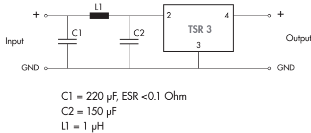
fig. 1 Positive output circuit
