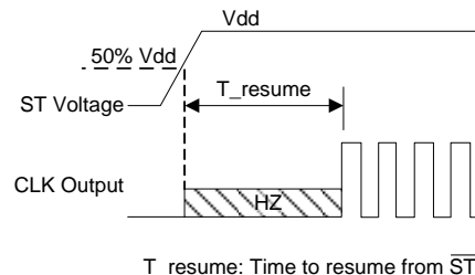
Figure 5. Standby Resume Timing ( \overline{\text{ST}} Mode Only)
