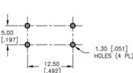
P.C. MOUNTING
