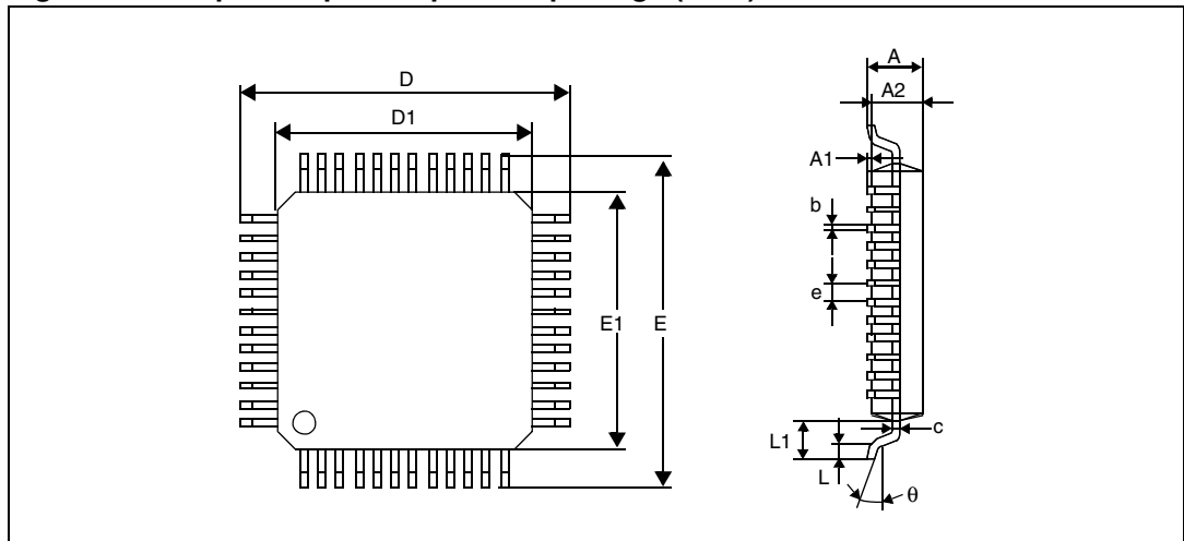
Figure 46. 48-pin low profile quad flat package (7 x 7)
