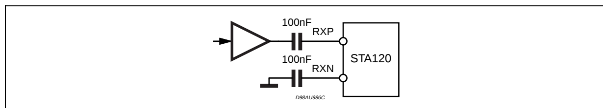
Figure 10. TTL/CMOS Interface
