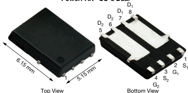
PowerPAK® SO-8 Dual
