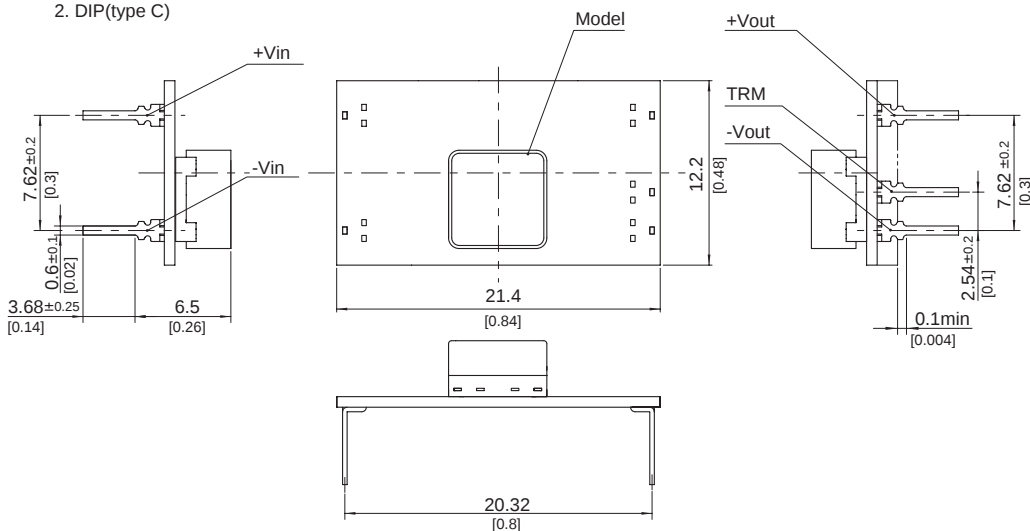
2. DIP(type C)
