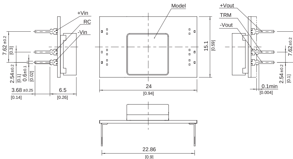
2. DIP(type C)
