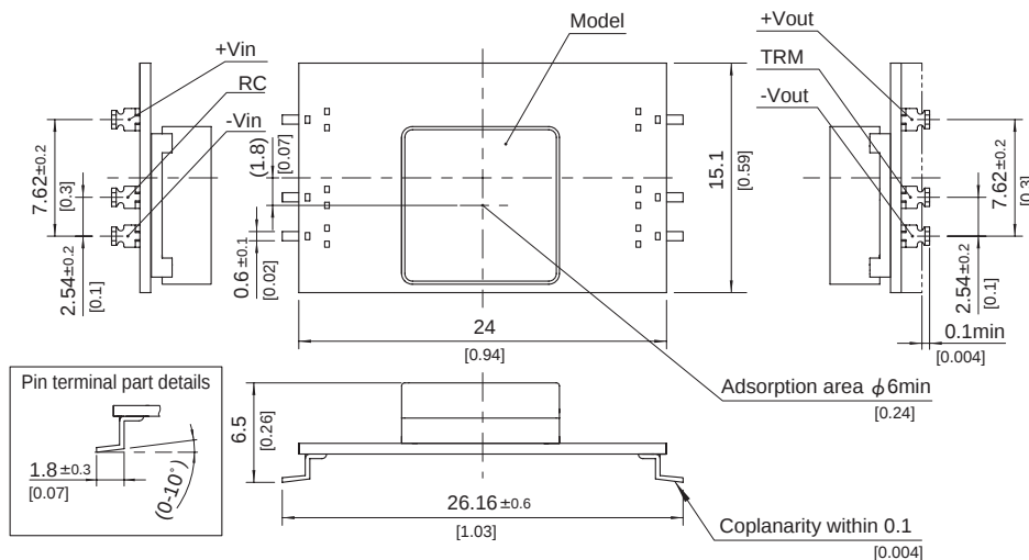
1. SMD(type B)
