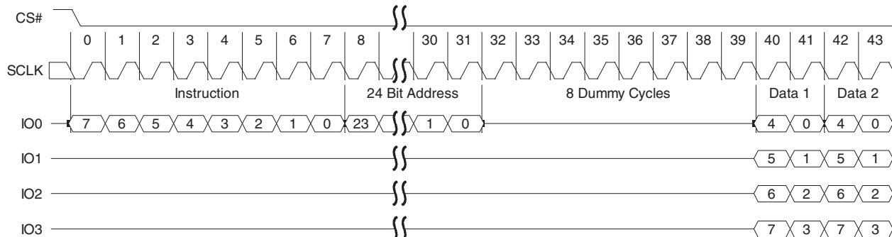
Figure 9.27 Quad Output Read (QOR 6Bh or 4QOR 6Ch) Command Sequence with Read Latency
