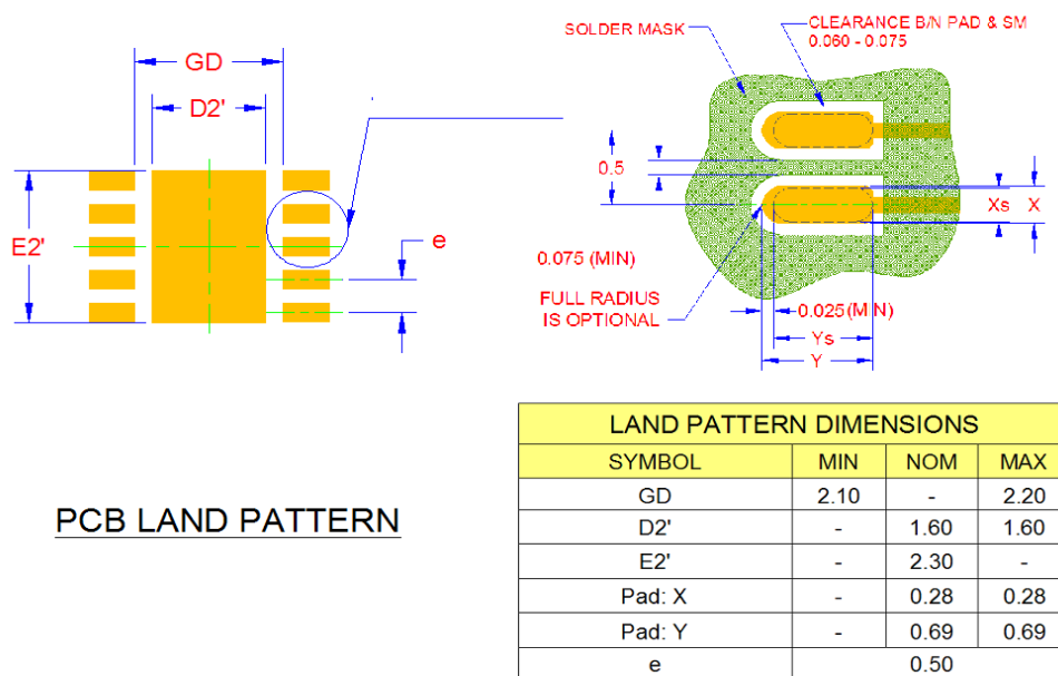
Figure 6.3 10-Pin DFN 3mm x 3mm PCB Footprint
