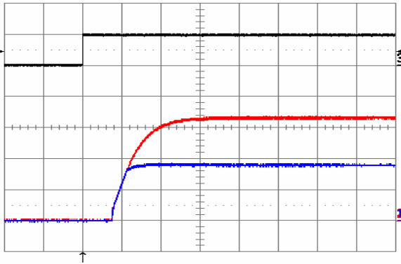
Fig. 22: Turn-on transient waveforms at no load current and Vin = 48 V, triggered via ON/OFF pin. Top trace: ON/OFF signal (5 V/div.). Bottom traces: Vout1 (blue, 1 V/div.), Vout2 (red, 1 V/div.). Time scale: 1 ms/div.
