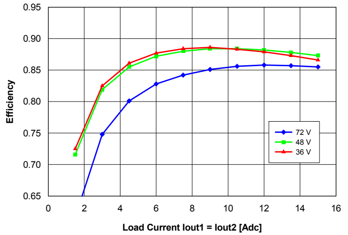
Fig. 21: Efficiency vs. balanced load current (lout1 = lout2) and input voltage for converter mounted horizontally with air flowing from pin 3 to pin 4 at a rate of 300 LFM (1.5 m/s) and Ta = 25°C.
