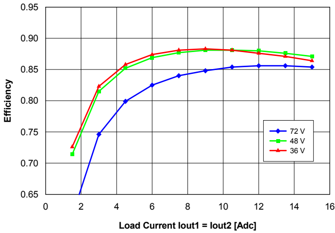
Fig. 20: Efficiency vs. balanced load current (lout1 = lout2) and input voltage for converter mounted vertically with air flowing from pin 3 to pin 1 at a rate of 300 LFM (1.5 m/s) and Ta = 25°C.
