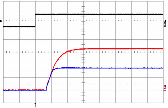
Fig. 23: Turn-on transient waveforms at full rated load current (resistive) and Vin = 48 V, triggered via ON/OFF pin. Top trace: ON/OFF signal (5 V/div.). Bottom traces: Vout1 (blue, 1 V/div.), Vout2 (red, 1 V/div.). Time scale: 1 ms/div.
