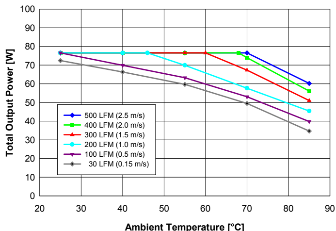
Fig. 1: Available output power vs. ambient air temperature and airflow rates for QD48T018033 converter mounted vertically with air flowing from pin 3 to pin 1, MOSFET temperature \leq 120^{\circ}\text{C} , V_{in} = 48\text{ V} and balanced load on both outputs ( I_{out1} = I_{out2} ).
