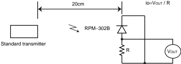
Fig.2 Measurement of standard transmitter proof reading.
