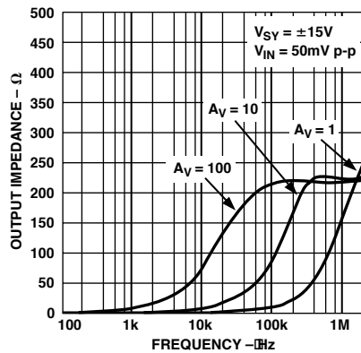
TPC 8. Output Impedance vs. Frequency
