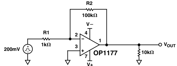
Figure 4. Test Circuit for Overload Recovery Time
