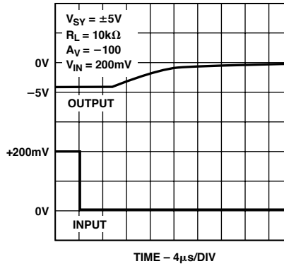
TPC 32. Positive Overtolerance Recovery
