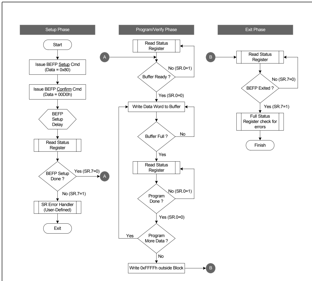
Figure 38: BEFP Flowchart
