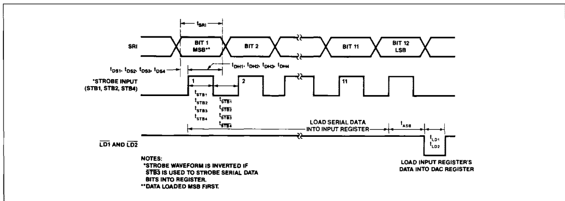
FIGURE 6: Timing Diagram
