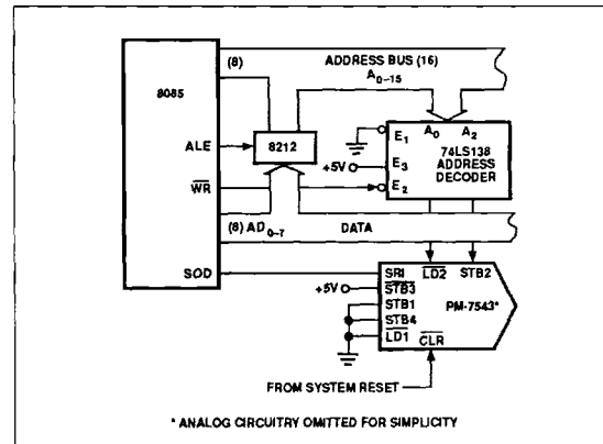
FIGURE 12: PM-7543 - 8085 Interface
