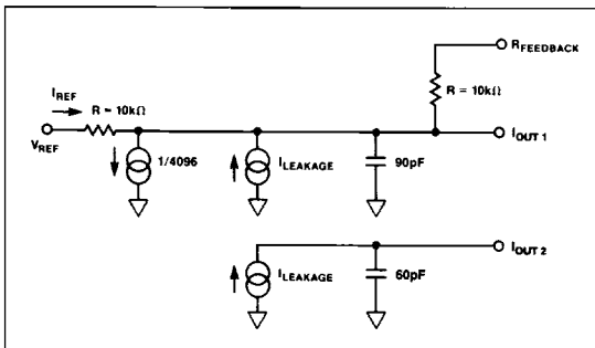
FIGURE 4: PM-7543 Equivalent Circuit (All Digital Inputs HIGH)
