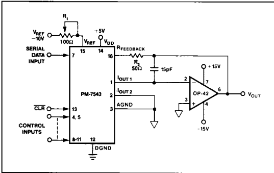
FIGURE 8: Unipolar Operation with Fast Op Amp and Gain Error Trimming (2-Quadrant)
