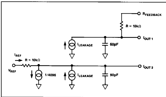
FIGURE 3: PM-7543 Equivalent Circuit (All Inputs LOW)
