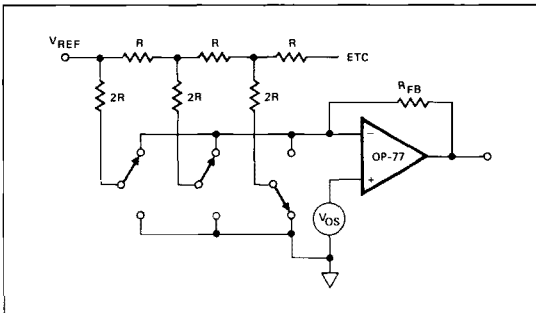
FIGURE 5: Simplified Circuit
