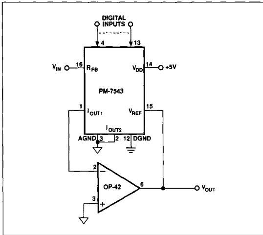
FIGURE 10: Analog/Digital Divider
