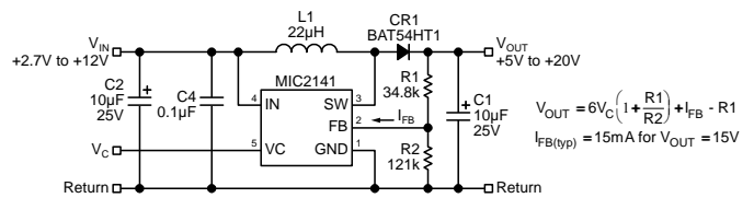
Figure 2. Gain-Boost Configuration
