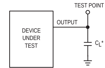
Figure 2. Test Circuit
