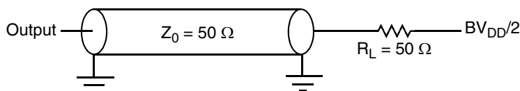
Figure 23. Local Bus AC Test Load
