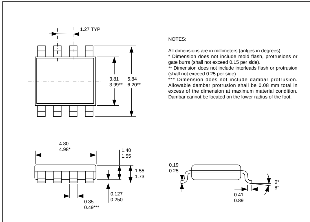
Figure 9: Package dimensions
