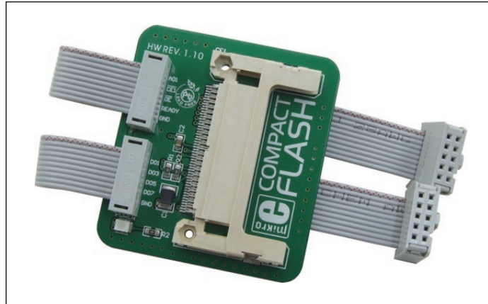
Figure 1: Compact FLASH additional board
