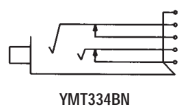
JACKS SCHEMATIC "N" SUFFIX DENOTES WELDED GOLD CONTACTS AND NICKEL-PLATED FRAME
