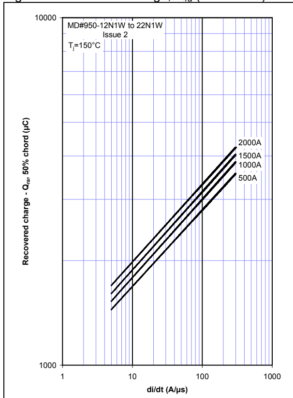
Figure 5 - Recovered charge, Q_{ra} (50% chord)
