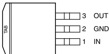
S-PAK-3 (R) MIC37150
