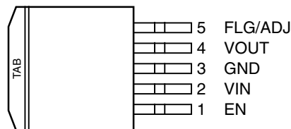
S-PAK-5 (R) MIC37151 MIC37152
