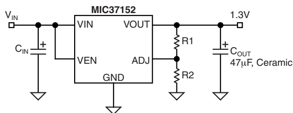
Adjustable Regulator
