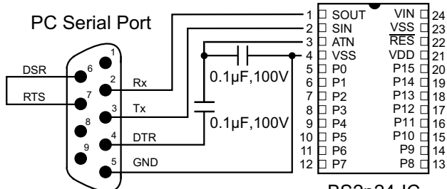
PC - to - BS2p24-IC connection
