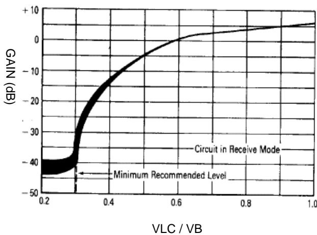
FIGURE 6 – RECEIVE ATTENUATOR versus VOLUME CONTROL
