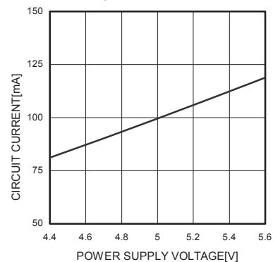
Fig.10 VCC Circuit current (Supply voltage dependence)
