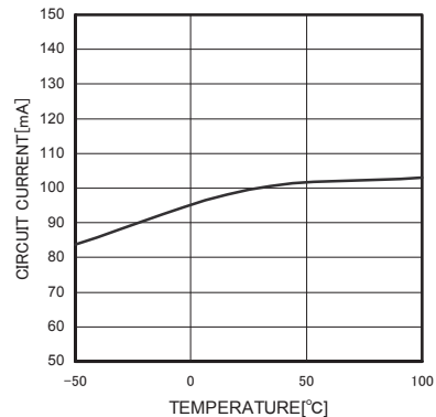
Fig.13 VCC Circuit current (Temperature dependence)
