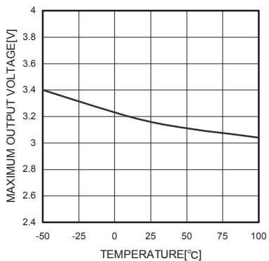
Fig.9 Maximum output voltage (Temperature dependence)
