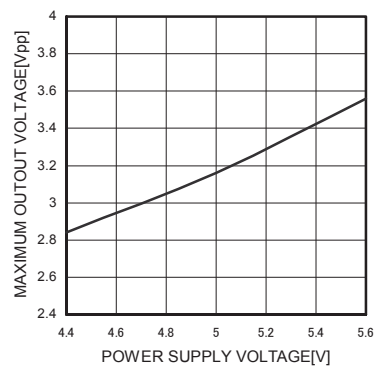
Fig.16 Maximum output voltage (Supply voltage dependence)
