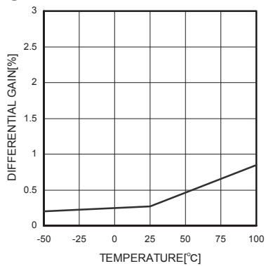
Fig.5 Differential Gain
