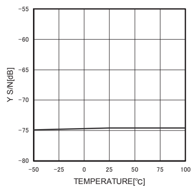
Fig.7 Y S/N ratio
