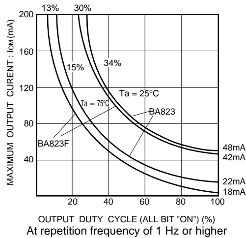
Fig. 7 Output conditions
