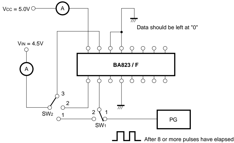
Fig. 2 I CC and I IH measurement circuit
