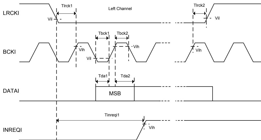
Figure 31. CD I/F Timing
