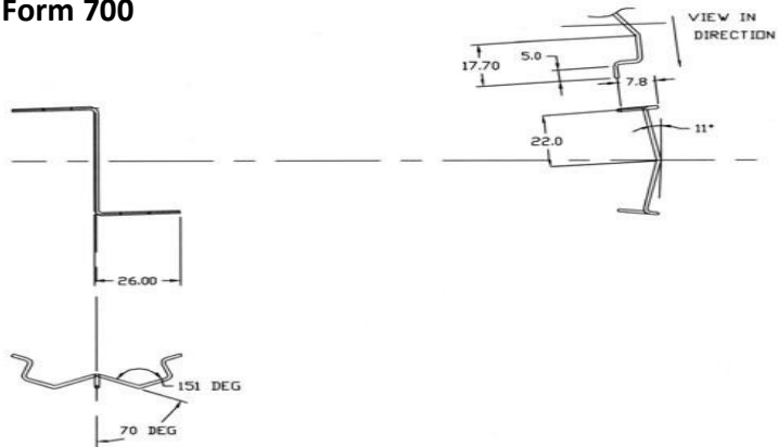
Wire Form 700
