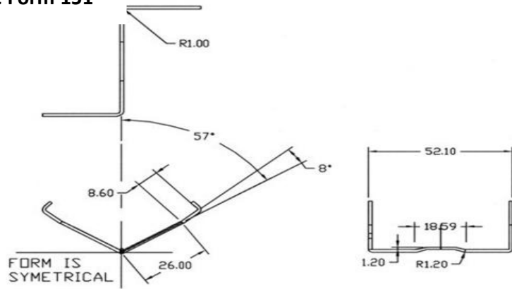
Wire Form 151
