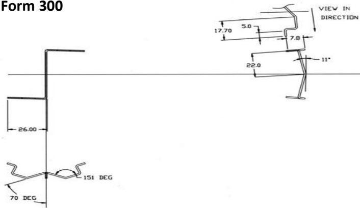
Wire Form 300
