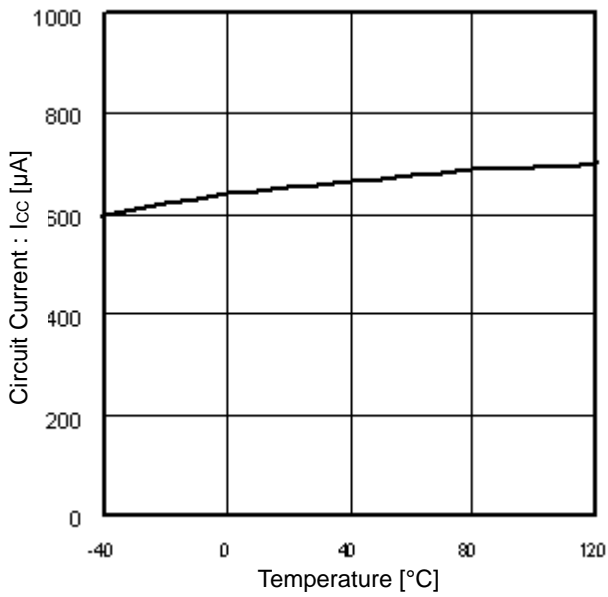
Figure 18. Circuit Current vs Temperature
