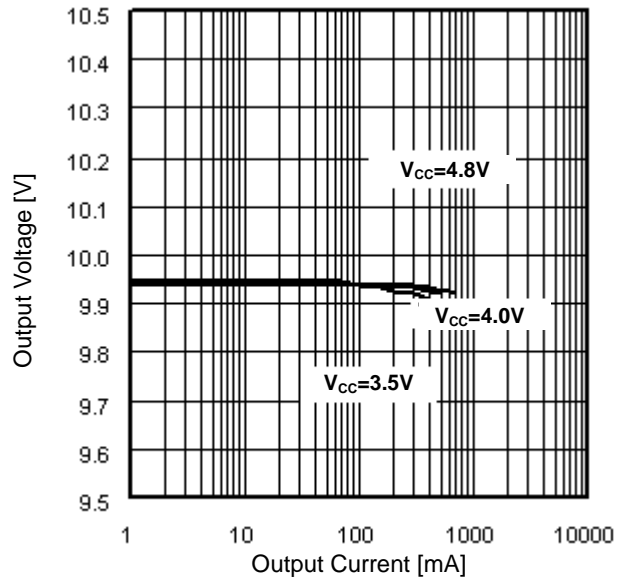
Figure 26. Load Regulation 2
