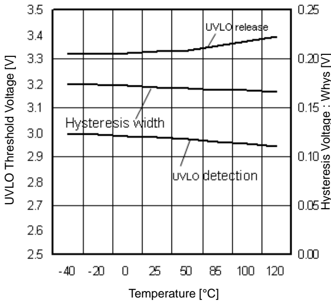
Figure 10. UVLO Threshold Voltage vs Temperature
