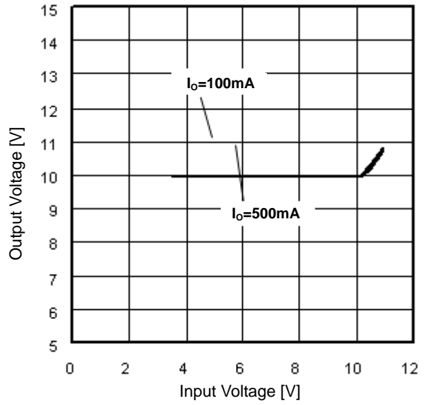
Figure 24. Line Regulation
