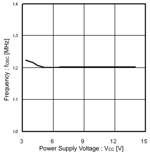
Figure 9. Frequency vs Power Supply Voltage
