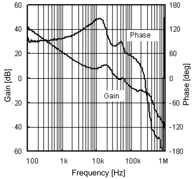
Figure 32. Frequency Response Property 6 ( V_{CC} = 8.4 V, I_o = 500mA )
