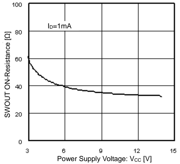
Figure 15. SWOUT ON-Resistance vs Power Supply Voltage
