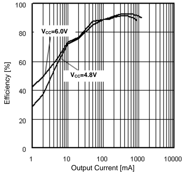
Figure 22. Power Conversion Efficiency 2
