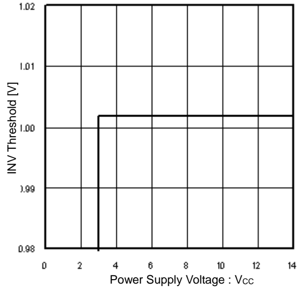
Figure 5. INV Threshold vs Power Supply Voltage
