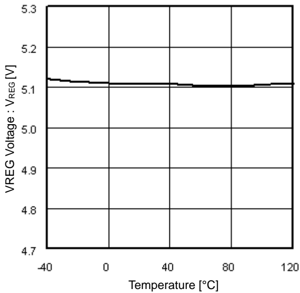
Figure 6. VREG Voltage vs Temperature
