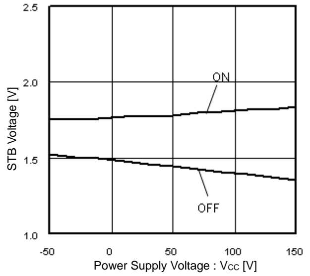
Figure 13. STB Voltage vs Power Supply Voltage
