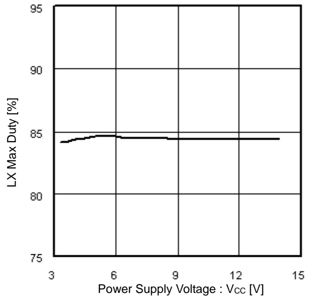
Figure 17. LX Max Duty vs Power Supply Voltage
