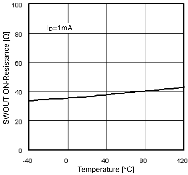
Figure 14. SWOUT ON-Resistance vs Temperature
