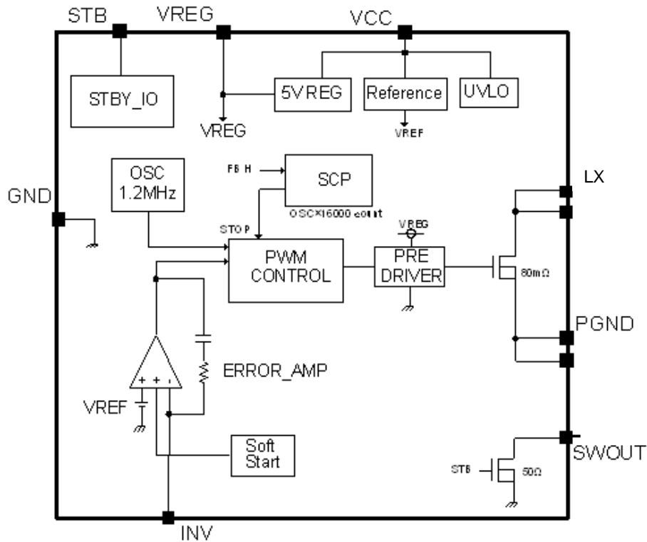
Figure 3. Block Diagram
