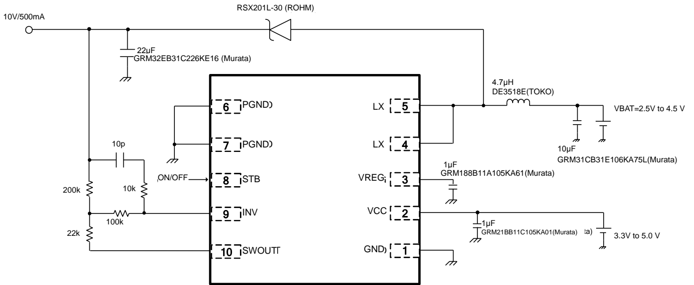
Figure 20. Reference Application Diagram
