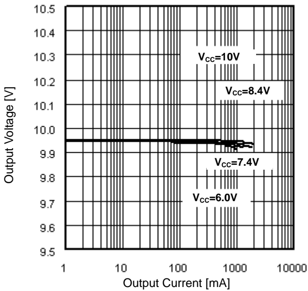
Figure 25. Load Regulation 1
