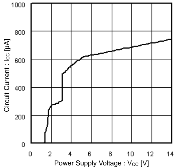
Figure 19. Circuit Current vs Power Supply Voltage
