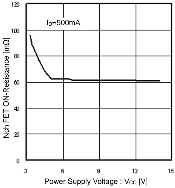
Figure 12. Nch FET ON-Resistance vs Power Supply Voltage
