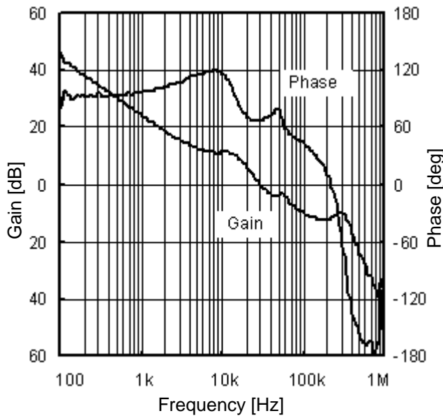
Figure 31. Frequency Response Property 5 ( V_{CC} = 6.0 V, I_o = 500mA )
