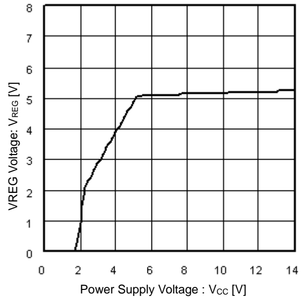
Figure 7. VREG Voltage vs Power Supply Voltage
